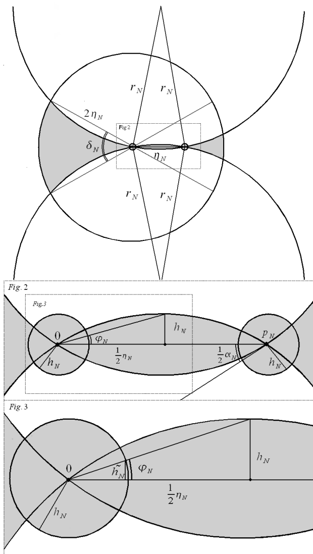
Figure 1. (See left.) A plane passing through two points 0 = \Gamma(0) and p_N = \Gamma(t_N) , located at the centers of two tiny shaded balls in the middle part of the picture. Big arcs represent the boundaries of two of the balls of radius r_N whose union is equal to the doughnut V_N . (Note: for \varepsilon small and N large, the ratio r_N/\eta_N is in fact much larger than the figure shows.) Later on, cf. (3.21) and (3.32), we prove that \gamma \cap B_{2\eta_N}(0) must be contained in
